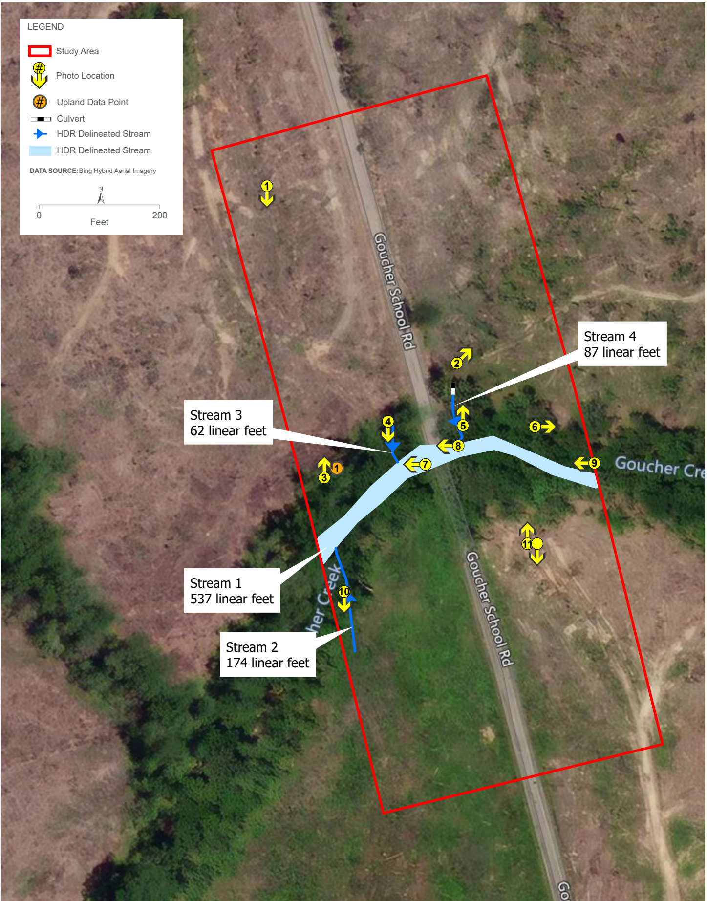
S-138 BRIDGE REPLACEMENT OVER GOUCHER CREEK Approximate Boundary of Waters of the U.S. Figure 4
